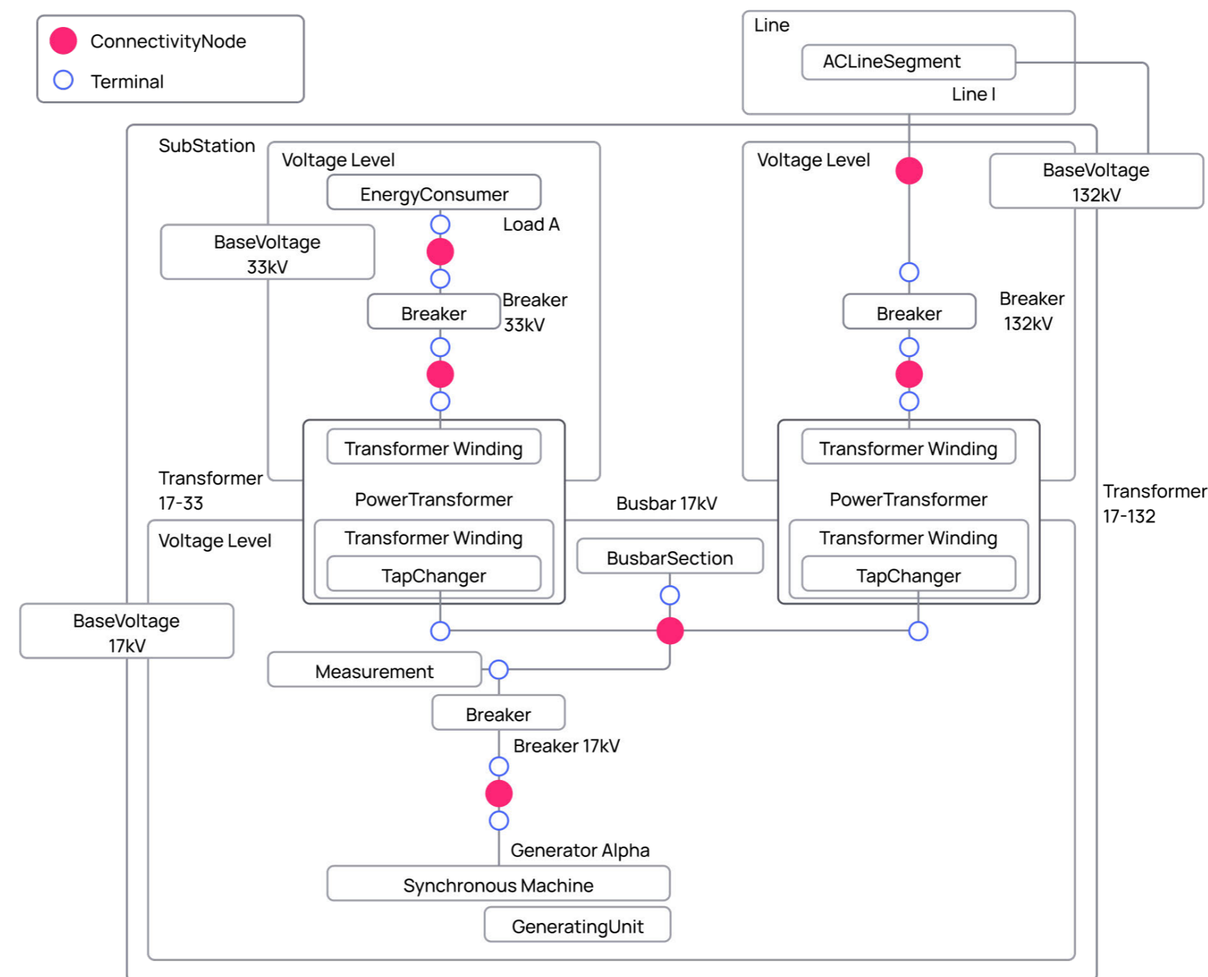
Figure 2: Example circuit with full CIM mappings (see Figure 3.13 in McMorrان, A.W. (2007). An Introduction to IEC 61970-301 & 61968-11: The Common Information Model.)
